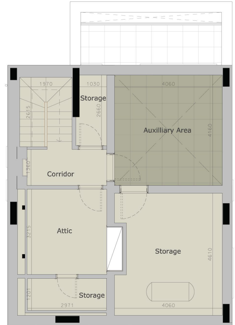
:2nd floor
