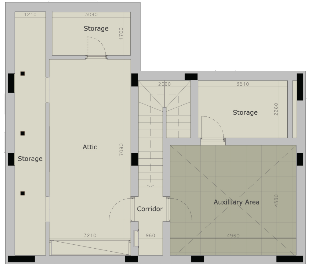
:2nd floor
